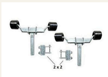
BOAT TRAILER ROLLER ASSEMBLIES Twin Front Adjustable Wobble Roller Assembly - 2" x 2"
