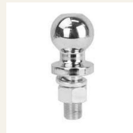
TOW BARS & ACCESSORIES Towball 50mm 3500kg Rated Chrome
